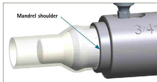
Figure 3. Correct installation of insert.
