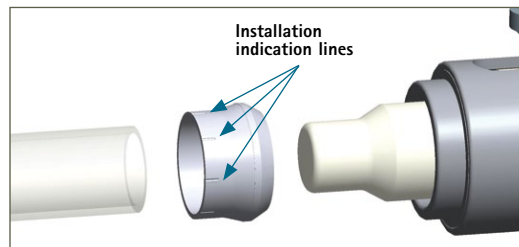
Figure 4. Incorrect installation of insert.
