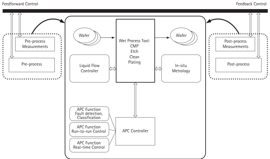
Figure 1: A generalized APC schematic to achieve better uniformity of process parameters by using liquid flow control.
