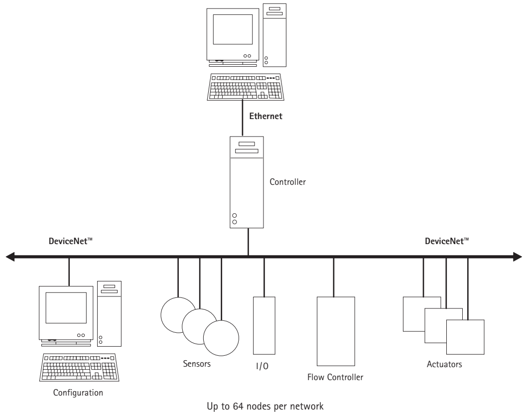
Figure 2: Typical DeviceNet™ communication network
