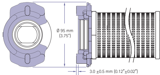
End View of Chemlock® Key on Cartridge
