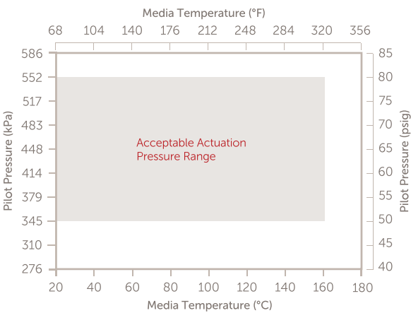
Normally Closed Valve Media Temperature vs. Actuator Pilot Pressure
