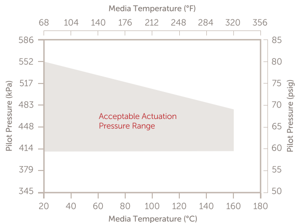
Normally Open Valve Media Temperature vs. Actuator Pilot Pressure
