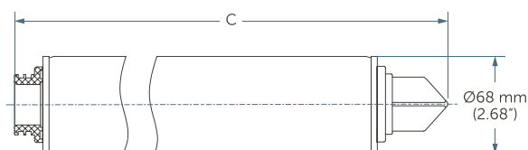
Ø68 mm Code 5 Filter
