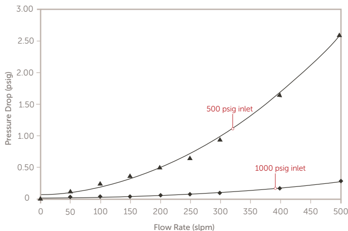
Pressure Drop Vs. Flow Rate HP3000, .003 µm Particle Filter (Nitrogen Gas)
