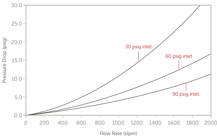
Pressure Drop Vs. Flow Rate MC14K, 0.003 µm Particle Filter, Tested in Nitrogen
