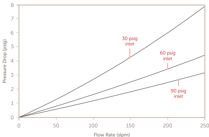
Pressure Drop vs. Flow Rate MC1500, 0.003 µm Particle Filter, tested in N 2
