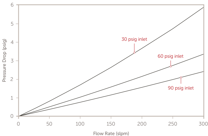
Pressure Drop Vs. Flow Rate MC2525-202F, .003 Micron, Nitrogen
