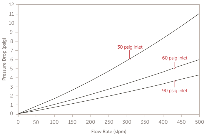
Pressure Drop vs. Flow Rate MC2550, 0.003 Micron Particle Filter, Nitrogen
