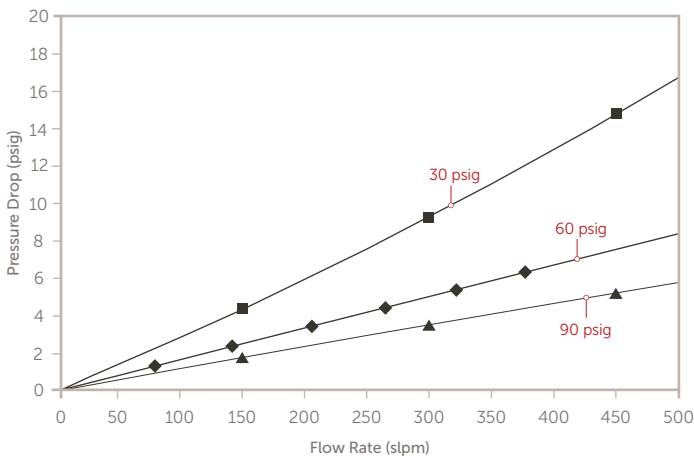
Pressure Drop Vs. Flow Rate MC3000, 0.003 Micron Particle Filter, nitrogen
