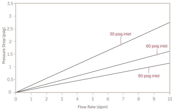
Pressure Drop Vs. Flow Rate MC45, 0.003 µm Particle Filter, Tested in N 2
