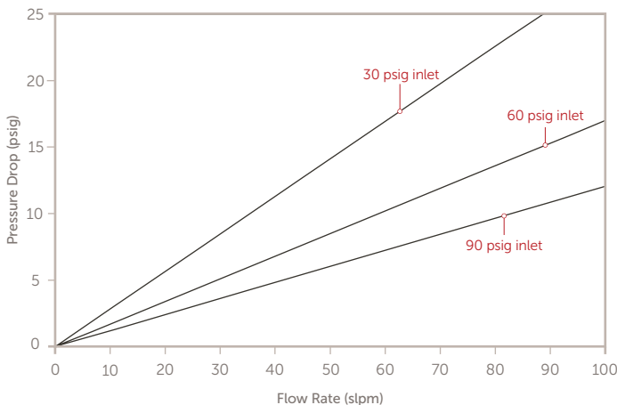
Pressure Drop Vs. Flow Rate MC500, 0.003 µm Particle Filter, Tested in N 2
