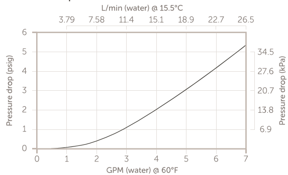
Pressure Drop vs. Water Flow
