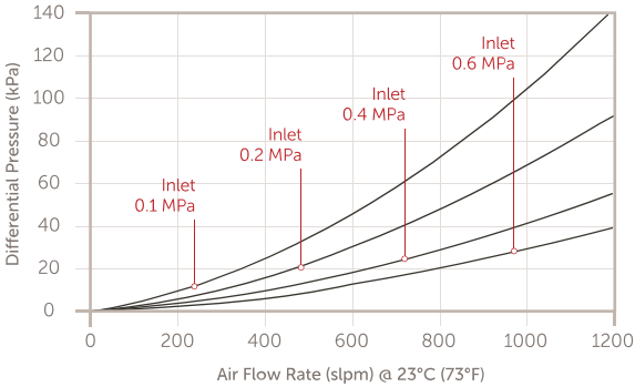
Lineagard MAX-FP Filters with ½" Fittings
