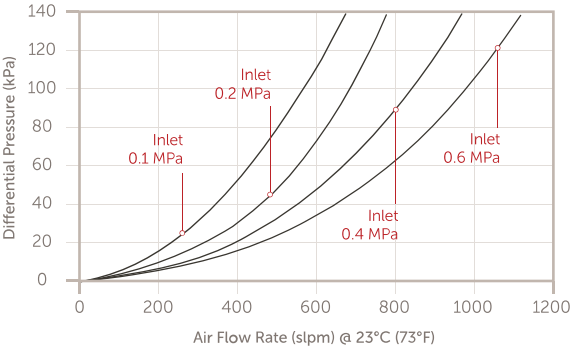
Lineagard MAX-FP Filters with ⅜" Fittings and ¼" NPT
