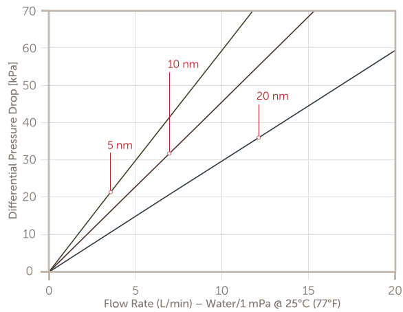
Microgard 10" Ø70 mm Cartridge Filters
