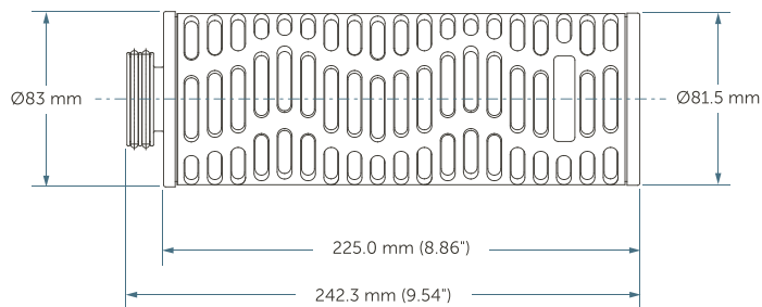
Microgard™ 10" Ø83 mm Cartridge Filter
