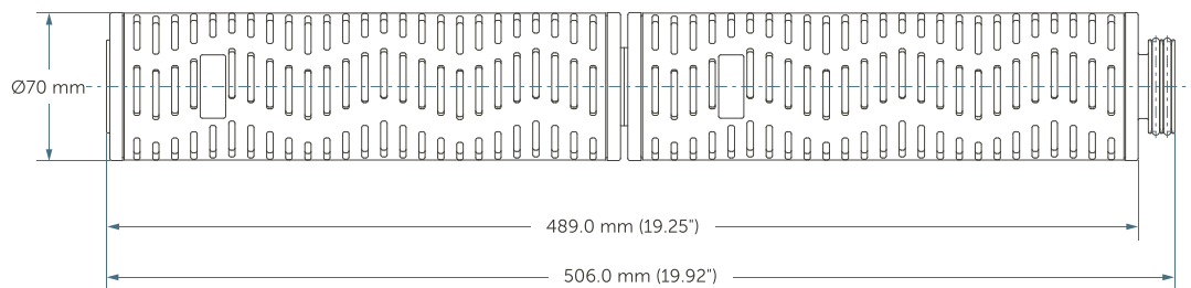
Microgard™ 20" Ø70 mm Cartridge Filter
