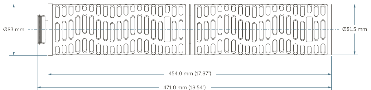
Microgard™ 20" Ø83 mm Cartridge Filter
