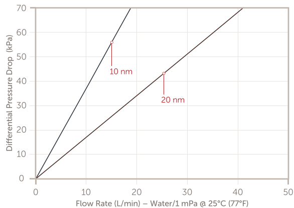
Microgard 10" Ø83 mm Cartridge Filters
