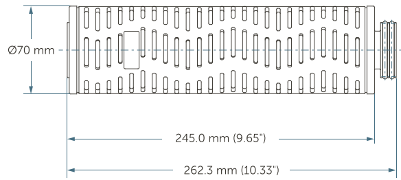
Microgard™ 10" Ø70 mm Cartridge Filter
