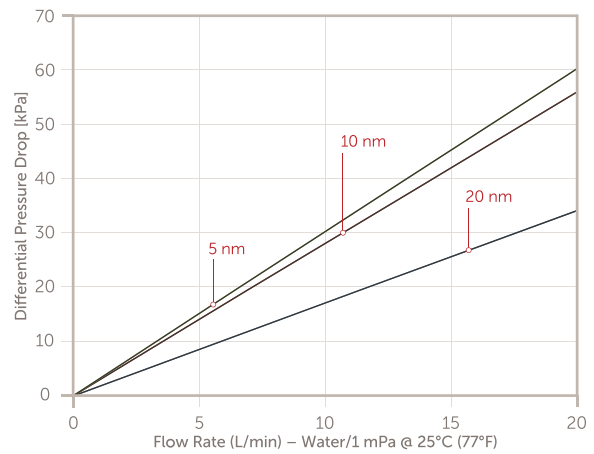
Microgard 20" Ø70 mm Cartridge Filters
