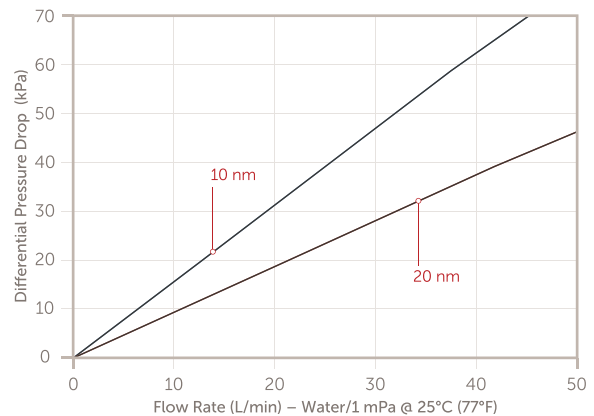
Microgard 20" Ø83 mm Cartridge Filters
