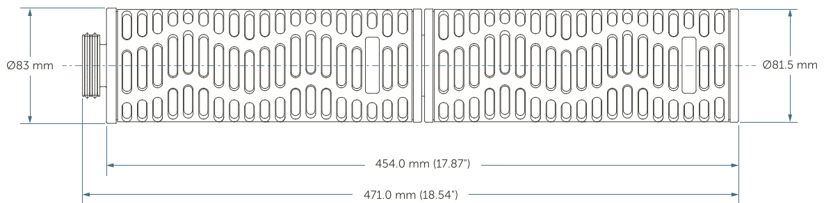
Microgard™ 20" Ø83 mm Cartridge Filter
