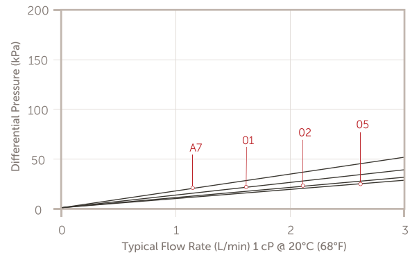
Planarcap NMB 5" Disposable Filters with 1/4" Inlet/Outlet Fitting (Ø89 mm)
