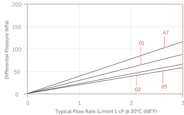
Planarcap NMB 2.5" Disposable Filters with 1/4" Inlet/Outlet Fitting (Ø89 mm)
