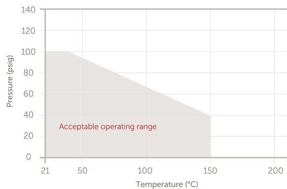
PrimeLock Fitting Sizes 1 1/2" and 40 mm Pressure vs. Temperature Rating
