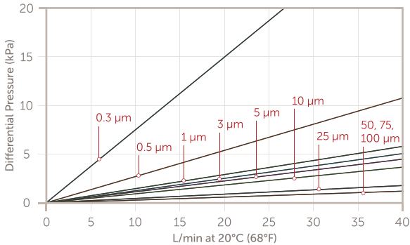
Processgard DEP 10" Cartridge
