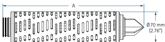
Ø70 MM CODE 5 FILTER
