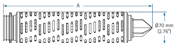
Ø70 MM CODE 7 FILTER
