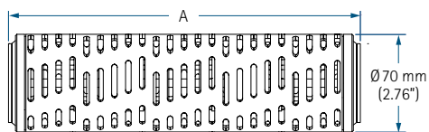
Ø70 MM CODE F FILTER
