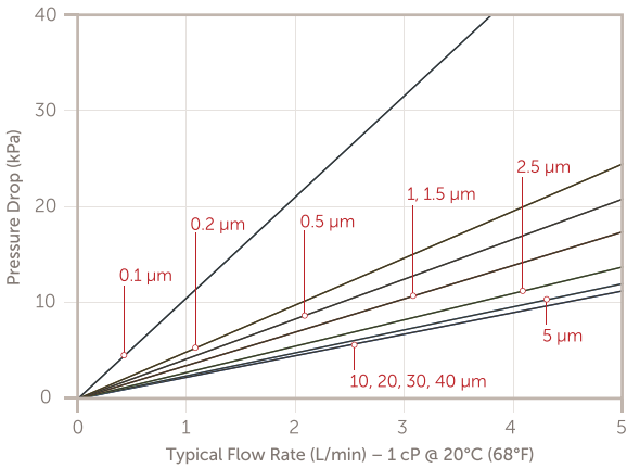
Processgard PDP Plus 2.5" Disposable Filters In/Out ¼ Compression Seal
