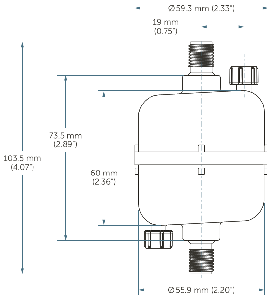
In/Out: ¼ Compression Seal
