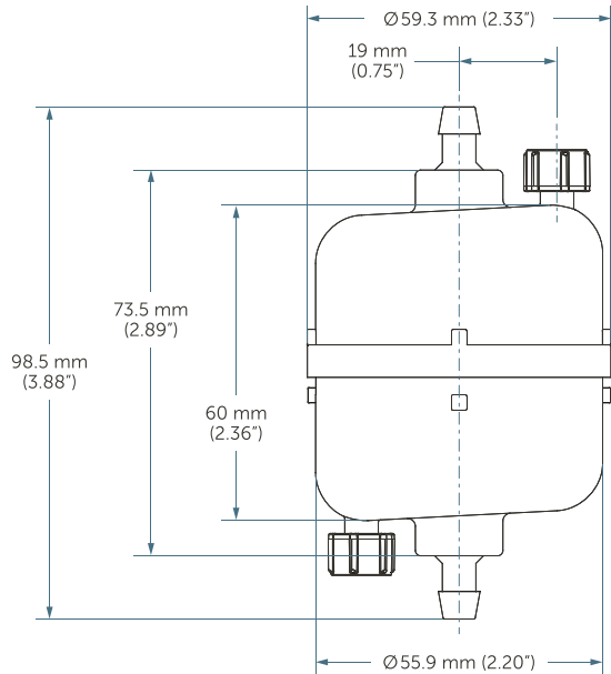
In/Out: ¼ Hose Barb
