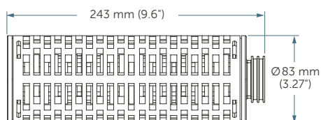
Ø83 mm Code 6 Filter
