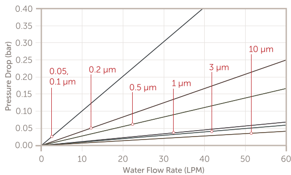
ProcessGard PTFE Plus, Code 0 10" cartridge
