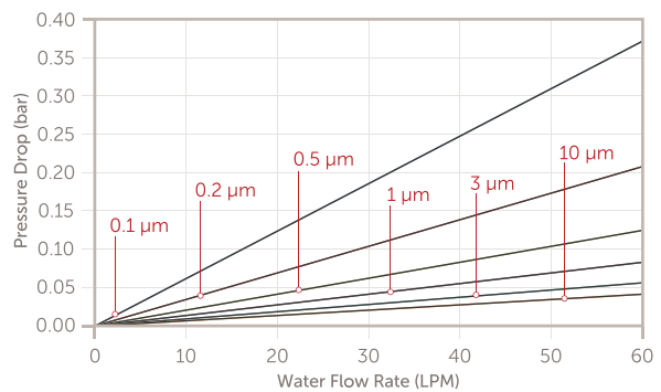
ProcessGard PTFE-HP Plus, Code 0 10" cartridge
