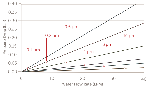
ProcessGard PTFE-HP Plus 4" cartridge
