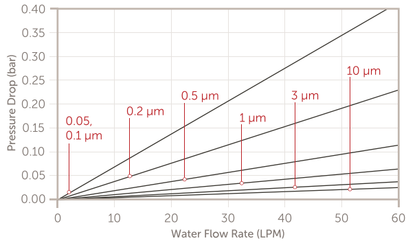
ProcessGard PTFE Plus, Code 6 10" cartridge
