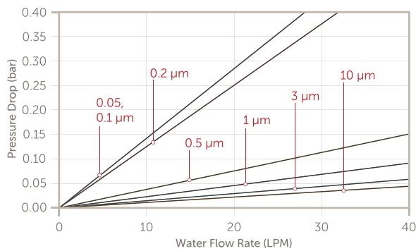
ProcessGard PTFE Plus 4" cartridge
