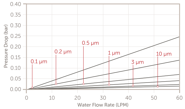
ProcessGard PTFE-HP Plus, Code 6 10" cartridge
