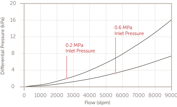
ProcessGard PTFE Plus Filters, 30" Code-O Air Flow Rate
