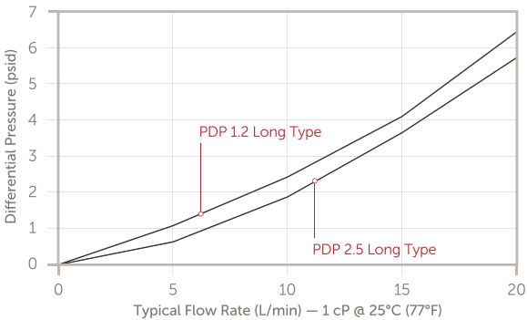
Savana 1-2-3 PDP Plus Long Disposable Filters
