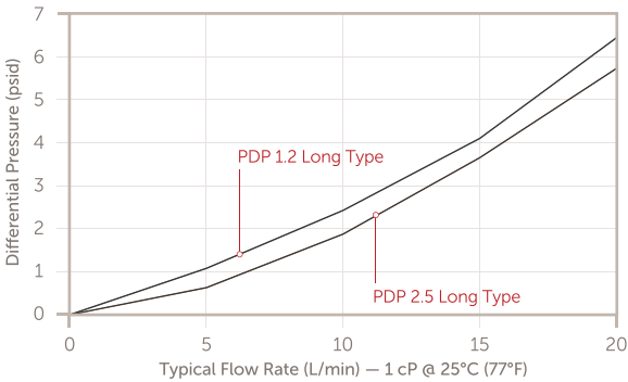
Savana 1-2-3 PDP Plus Long Disposable Filters
