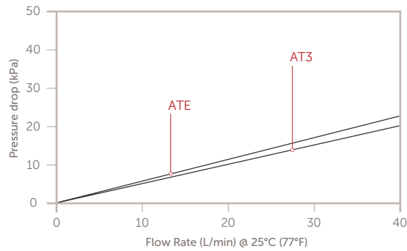
Torrento X 2 nm 20" Cartridge Filters Pressure Drop vs Flow Rate, DI Water
