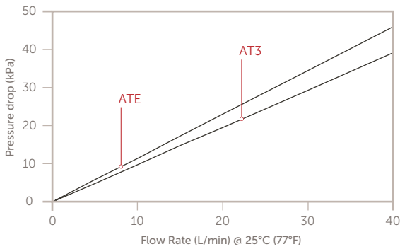
Torrento X 2 nm 10" Cartridge Filters Pressure Drop vs Flow Rate, DI Water
