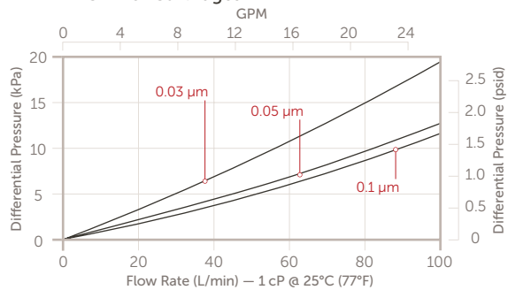
Trinzik HCM 30" Cartridges
