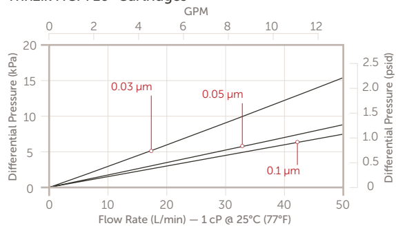
Trinzik HCM 20" Cartridges
