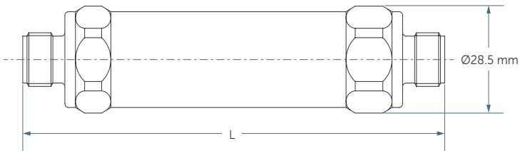
WGFG02PS1: L = 115.5 mm (4.55") WGFG32PS1: L = 119.3 mm (4.70")
