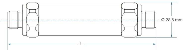
YY5002PR1 (6.35 mm (1/4") 接続) : L = 127.0 mm YY5032PR1 (12.7 mm (1/2") 接続) : L = 133.5 mm
