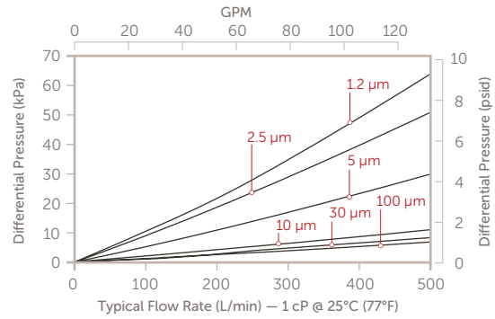
Panelgard Ex PP Filters
