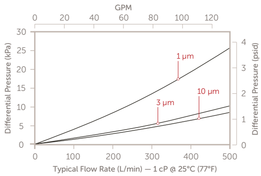
Panelgard Ex THF Filters
