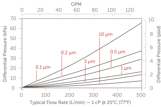
Panelgard Ex THP Filters
