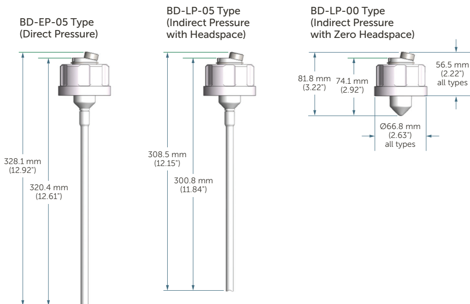
BrightPak Bottle with Connector and Diptube (Maximum Height including Fitting)
