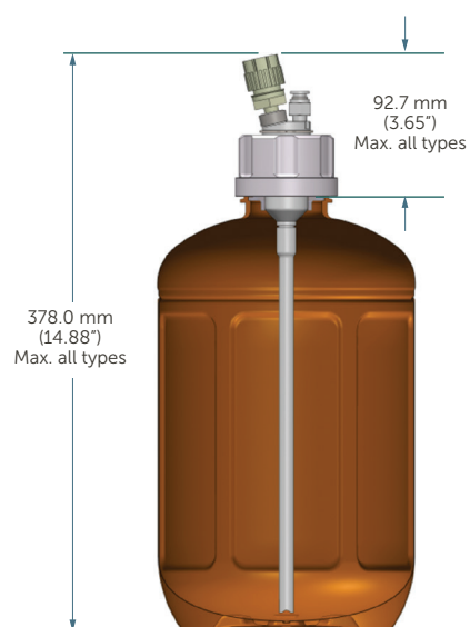
BrightPak Bottle with Connector and Diptube (Maximum Height including Fitting)
