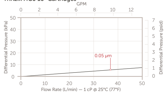
Trinzik HCO 20" Cartridges
