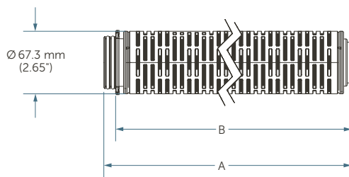
Code 6 - 226 Flat
