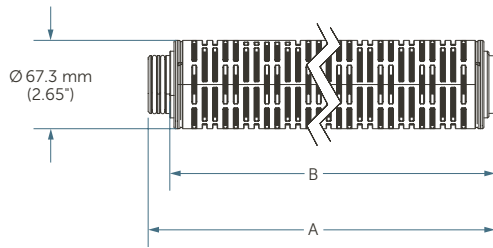
Code 0 - 222 Flat
