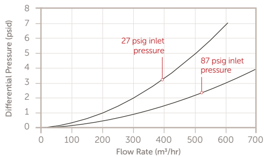
Savana 20" Cartridge Filter
