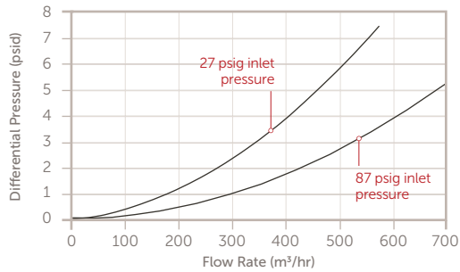
Savana 10" Cartridge Filter
