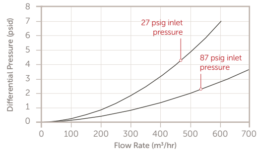
Savana 30" Cartridge Filter
