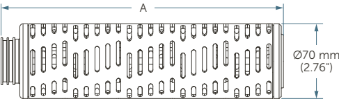
Ø70 mm Code 0 Filter
